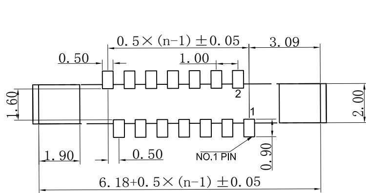
PCB BOARD LAYOUT
