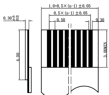
RECOMMENDED FPC/FFC DIM
